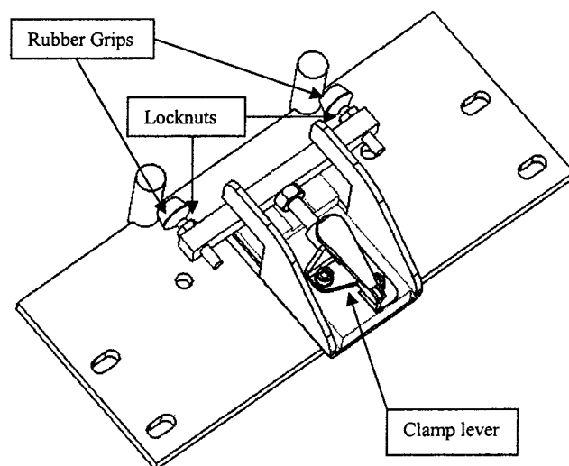
Fig 3: Adjustment
