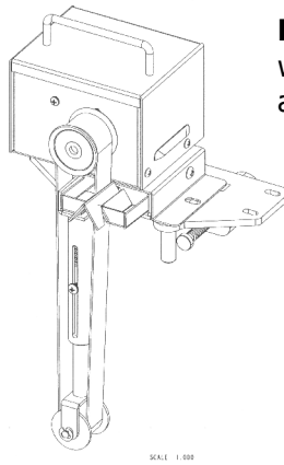
Fig.3: Adjustments
