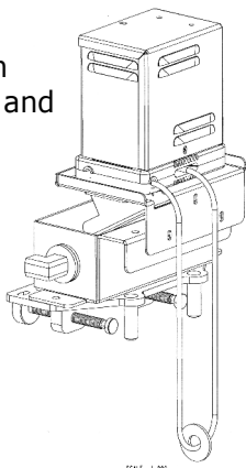
Fig.2: Mounting Holes
